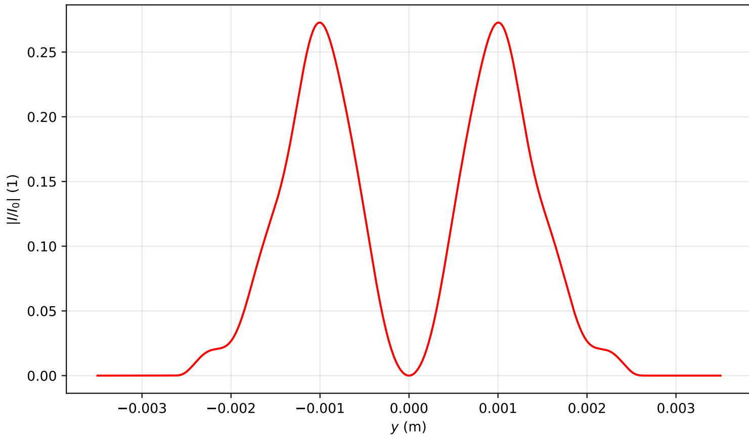
Intensity profile I(x=0, y, z=3.901)/I_0 , P_{in}=2.0P_{cr} , artificial time
